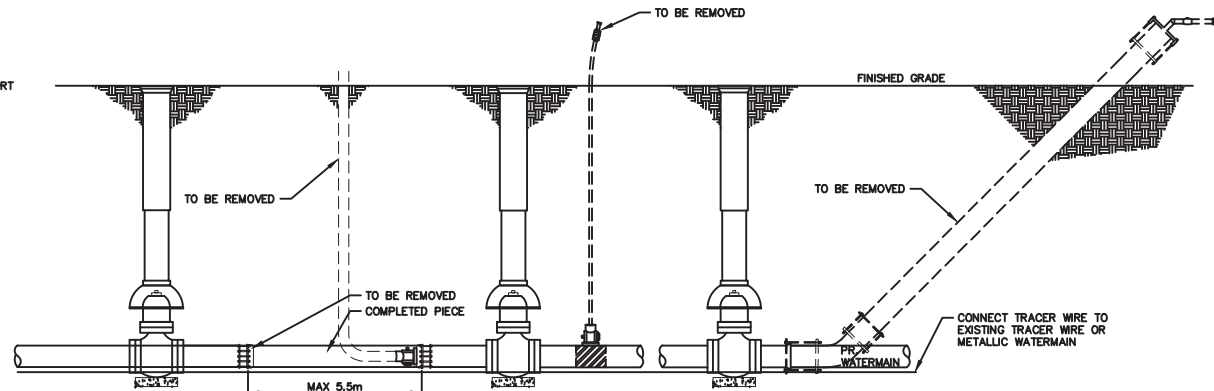
WATERMAIN COMPLETION ASSEMBLY
