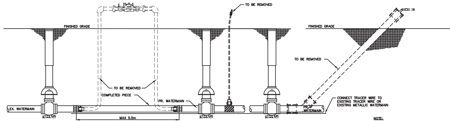
WATERMAIN COMPLETION ASSEMBLY
